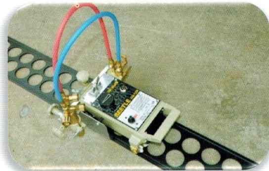
Complete Set With Cutting Torch Body , Cutting Nozzles & Standard 6 Feet Rail
